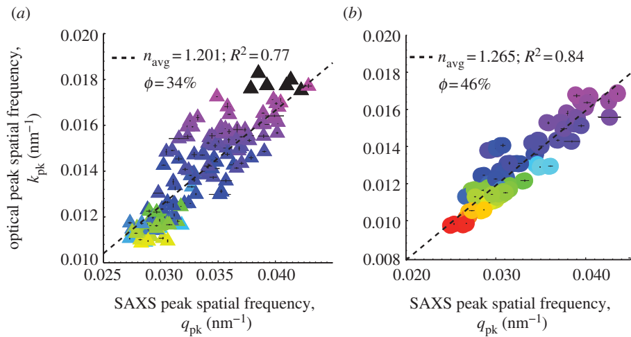
Figure 8. Regression plots of the primary optical peak hue from normal incidence reflectance measurements expressed as peak spatial frequency ( k_{pk} = 2\pi/\lambda_{pk} ) against the dominant spatial frequency of structural correlations ( q_{pk} ) measured using SAXS for (a) channel- (shaded triangles) and (b) sphere-type (shaded circles) nanostructures. For both nanostructural classes, the size of the nanostructural periodicity measured by SAXS strongly predicts, i.e. scales with the measured primary peak hue, demonstrating that the underlying barb nanostructures are tuned to produce the observed structural colours. The inverse of twice the slope of the regression yields n_{avg} , the average or effective refractive index (and hence \phi , the keratin volume fraction) for each class of nanostructure. The estimated n_{avg} and \phi for sphere nanostructures on the whole (1.265, 46%) is significantly higher than that for channel morphologies (1.201, 34%) and congruent with predictions of the phase separation hypothesis. The colour of each triangle or circle is coded to the approximate colour of the corresponding feather (UV colours in black). The vertical and horizontal lines at each data point indicate the standard error of the mean (s.e.m).
